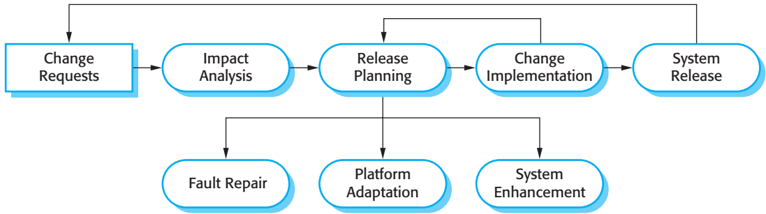
Figure 9.4 The software evolution process
