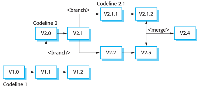
Figure 25.9 Branching and merging
