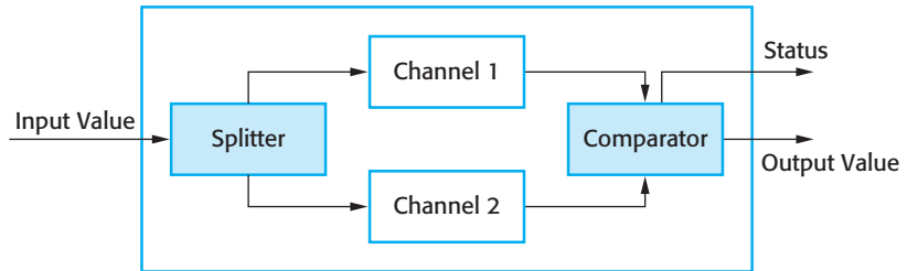
Figure 13.4 Self-monitoring architecture
