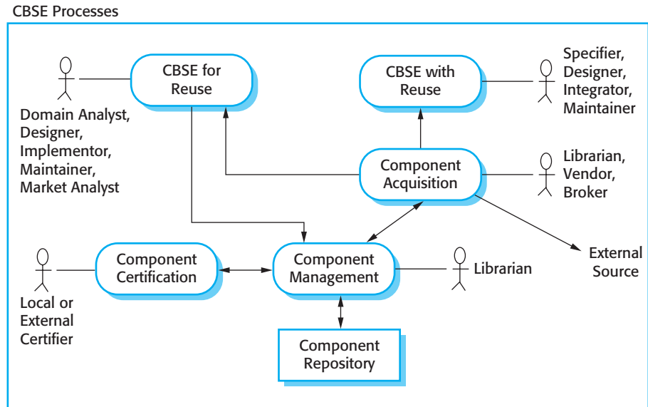
Figure 17.6 CBSE processes
