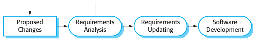
Figure 9.5 Change implementation
