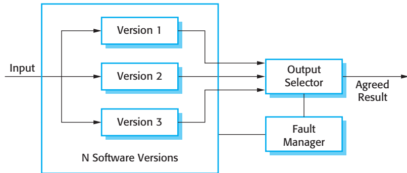
Figure 13.7 N-version programming
