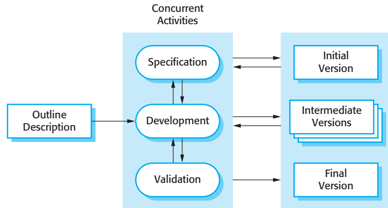
Figure 2.2 Incremental development
