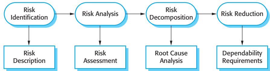
Figure 12.1 Risk-driven specification
