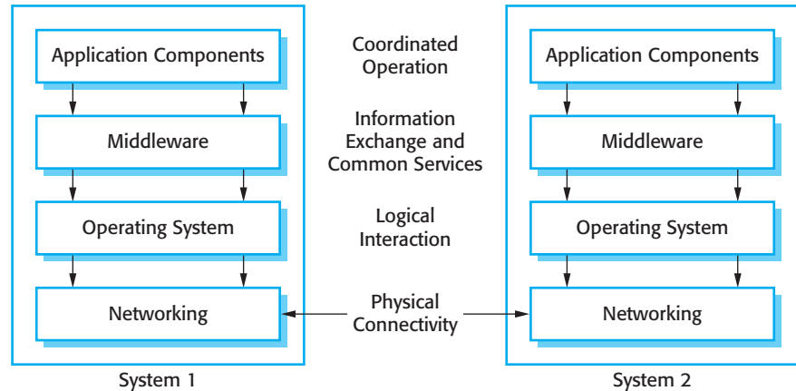
Figure 18.3 Middleware in a distributed system
