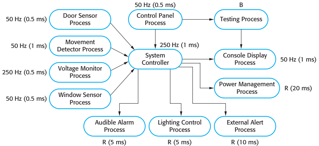
Figure 20.16 Alarm process timing
