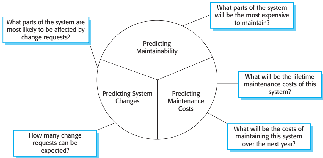
Figure 9.10 Maintenance prediction
