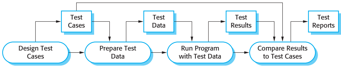
Figure 8.3 A model of the software testing process
