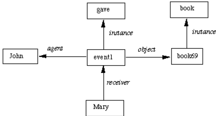
Fig. A Semantic Network for a Sentence
